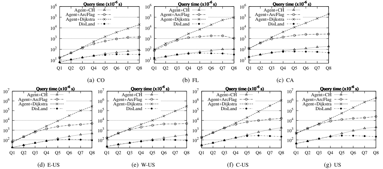
Figure 10. Performance evaluation w.r.t. distance queries
